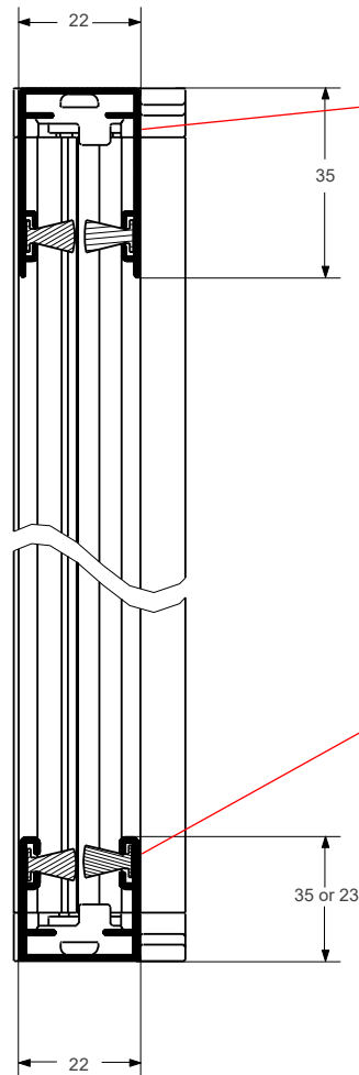
Vertical Section
