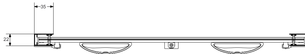
Horizontal Section - cassette not shown
