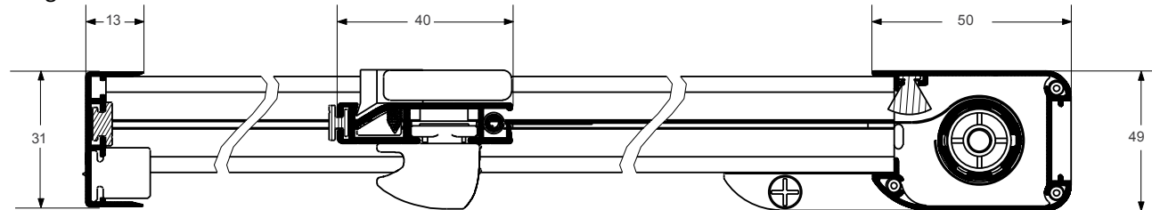
Magnetic Profile
